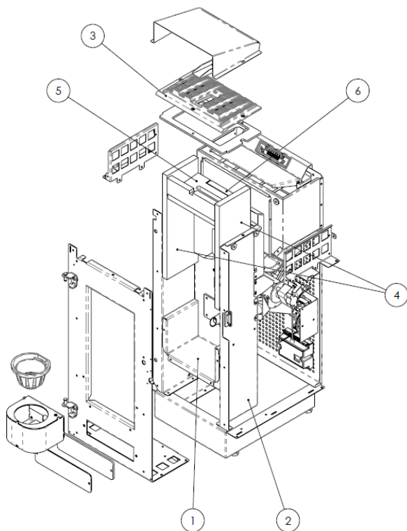
Exploded view of VISION ERMETICA stove combustion chamber and parts
